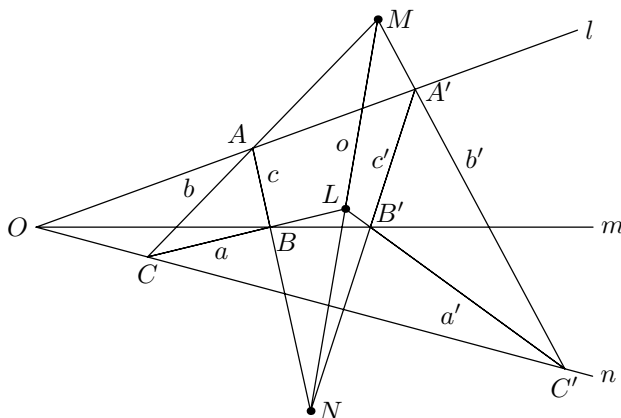
Figure 5.2 Desargues' dual
