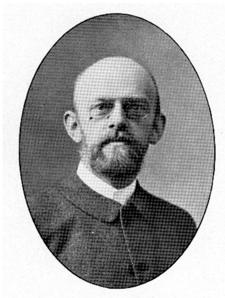
Figure 23.1 Hilbert
