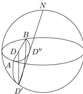
Figure 25.2 Poincaré's projections
