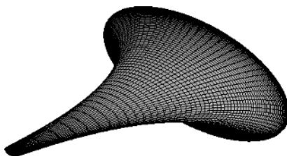
Figure 11.1 A pseudosphere
