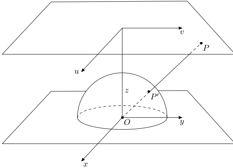
Figure 19.1 Geodesic projection (1)
